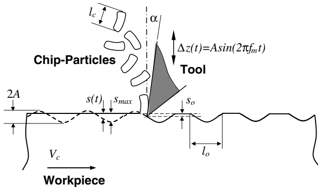
Figure 1. Plane-strain machining with and without modulation. A workpiece moving at a velocity V_c is traversed by the sharp cutting edge of a wedge-shaped tool inclined at rake angle, \alpha . In conventional machining, the tool is engaged at a preset depth, s_0 (undeformed chip thickness). In modulation-assisted machining (MAM), a sinusoidal motion \Delta z(t) is superimposed on to the tool in the direction of undeformed chip thickness. When the modulation amplitude, A , is sufficiently high, the chips form as discrete particles with undeformed length, l_0 , and undeformed thickness, s_{\max} , with one particle being created in every cycle of the modulation.
