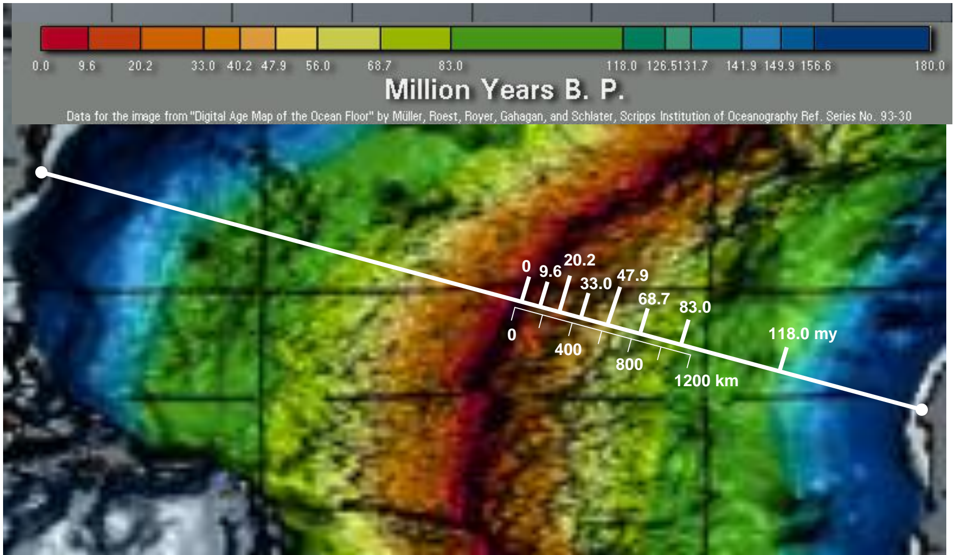
Ocean crust ages for a portion of the North Atlantic Ocean (from http://www.ngdc.noaa.gov/mgg/image/crustageposter.gif ). Zoom to 130% to enlarge scale to 0.5 cm = 100 km for convenient location of distances along the profile.
