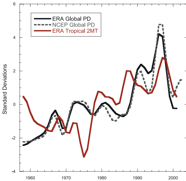
Figure 2. ERA-40-derived global PD (black curve), NCEP-derived global PD (dashed curve) and ERA-40 mean annual tropical 2MT (red curve). Tropical 2MT is averaged annually from 30 degrees north to 30 degrees south globally, and all curves are normalized with the respective standard deviations of the detrended time series. The correlation between ERA-40 PD and ERA-40 2MT is r^2 = 0.34 .
