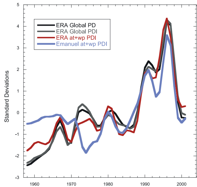
Figure 1. PD quantities for the ERA-40 project period, 1958–2001. ERA-40-derived quantities include global PD (black curve), global PDI (gray curve), and PDI for the Atlantic and northwestern Pacific regions (red curve). Also shown is the Atlantic and northwestern Pacific PDI derived from Emanuel [2005] data and filtered using the technique discussed in the methods section (blue curve). All curves are normalized with the respective standard deviations of the detrended time series.
