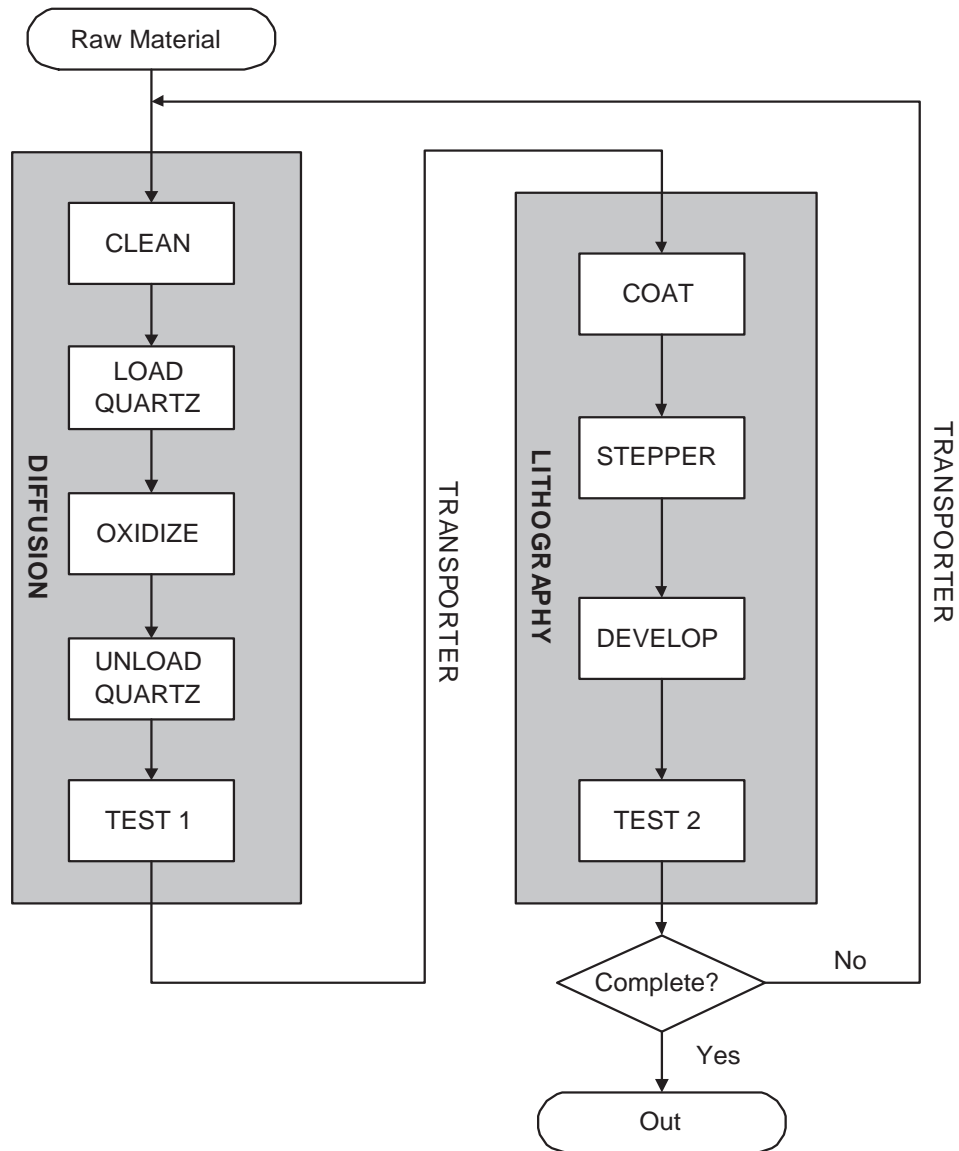
Figure 8: Production Process of the Semiconductor Manufacturing Case Study
