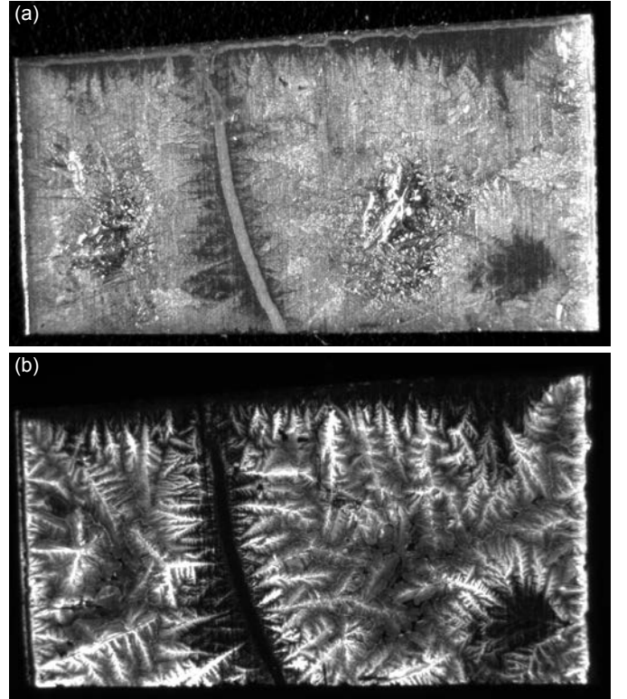
Fig. 1. The upper image (a) shows a room-light image of the thin-film InP sample. The lower image (b) shows the PL image. The sample is 1 cm wide.
