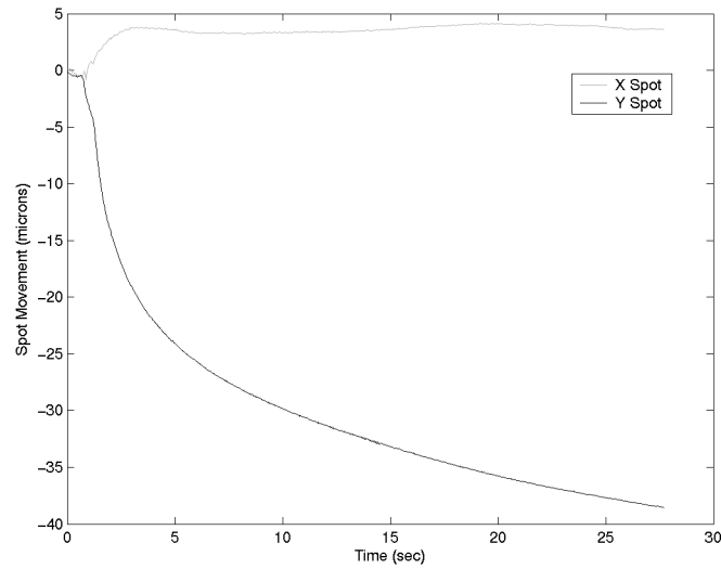
FIGURE 9: SPOT MOTION WITH FORCE ACCOMMODATION TURNED ON.
