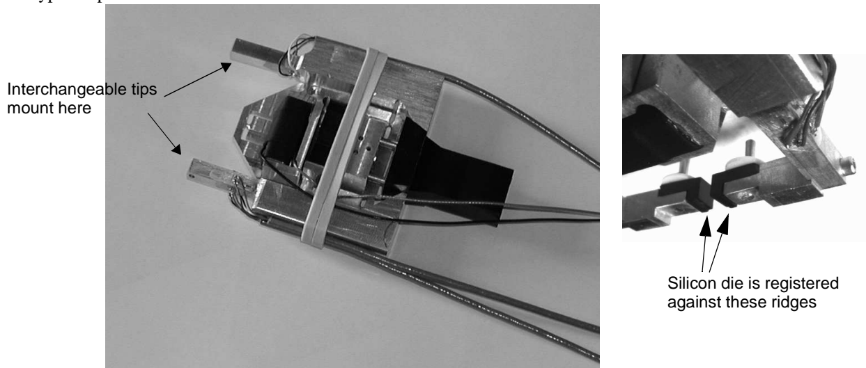
FIGURE 4: THE FABRICATED MICRO/MACRO GRIPPER. OVERALL DIMENSIONS ARE APPROXIMATELY 50 MM WIDE BY 75 MM LONG. THE INSET SHOWS THE MOUNTING OF THE SILICON TIPS.
