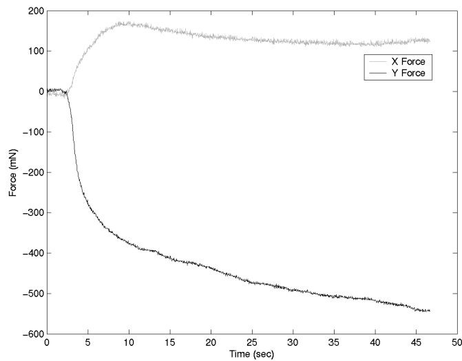
FIGURE 8: FORCE RESPONSE OF THE FIRST TRIAL. THE ONLY FORCE ACCOMMODATION IS PASSIVE FLEXING OF THE STRUCTURE.
