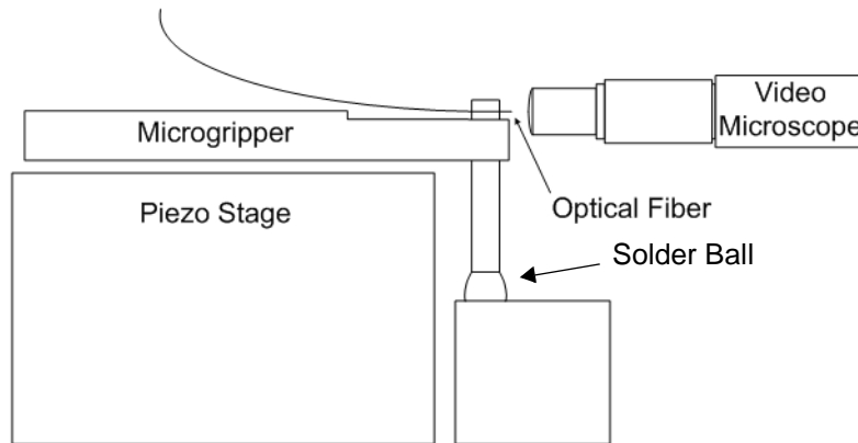
FIGURE 5: EXPERIMENTAL APPARATUS WITH 3-AXIS PIEZO STAGE AND SPOT TRACKING.
