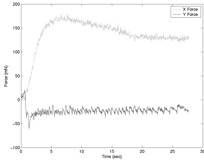
FIGURE 10: FORCE RESPONSE IN X AND Y WITH Y FORCE CONTROL TURNED ON.
