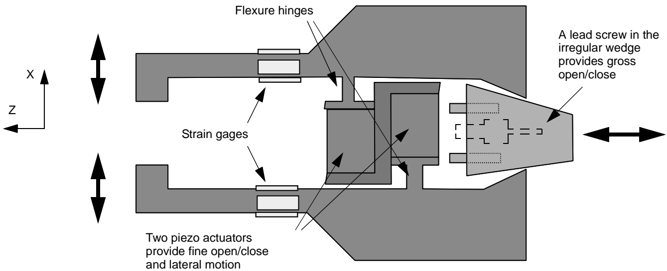
FIGURE 2: SCHEMATIC DRAWING OF THE MICRO/MACRO ACTUATION OF THE GRIPPING DEGREE OF FREEDOM. THREE ACTUATORS PROVIDE GROSS/FINE OPENING AND CLOSING OF THE TIPS PLUS LATERAL MOTION.
