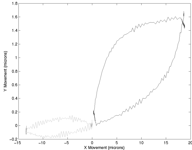
FIGURE 6: RELATIVE MOVEMENT OF THE LEFT AND RIGHT FINGERTIPS DURING FREE GRIPPING MOTIONS. (LEFT FINGER IS ON THE RIGHT FROM THE SPOT TRACKER VANTAGE POINT.)
