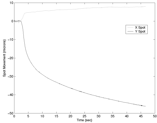
FIGURE 7: MOTION OF THE SPOT IN X AND Y AS THE SOLDER COOLS WITH NO ACTIVE FORCE ACCOMMODATION.
