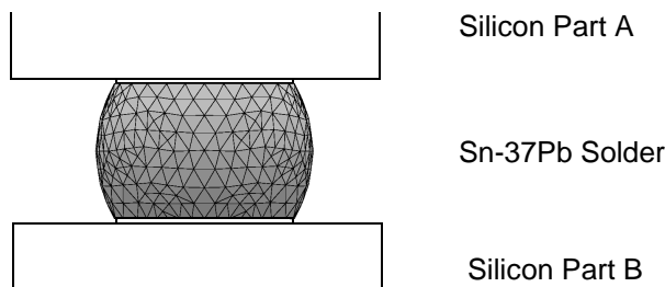
FIGURE 1: SOLDER BALL ATTACHMENT OF METALLIZED SILICON PIECES. (RESULTING SOLDER SHAPE SIMULATED WITH SURFACE EVOLVER 12 .)
