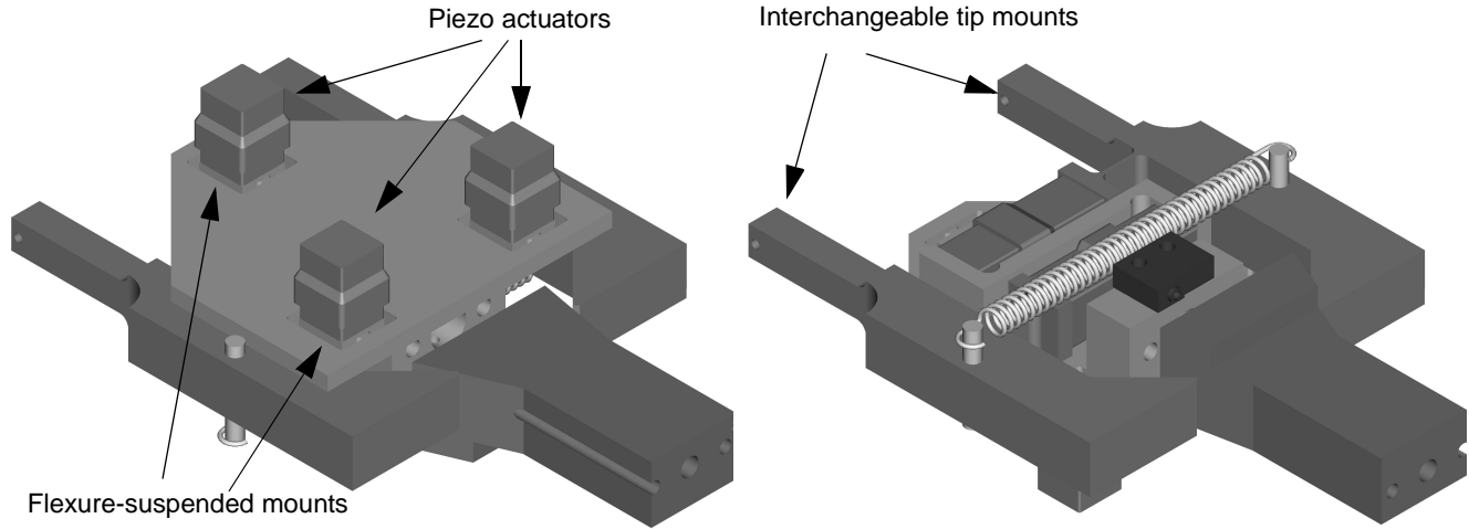
FIGURE 3: BOTTOM AND TOP CAD VIEWS OF THE MICRO/MACRO GRIPPER.
