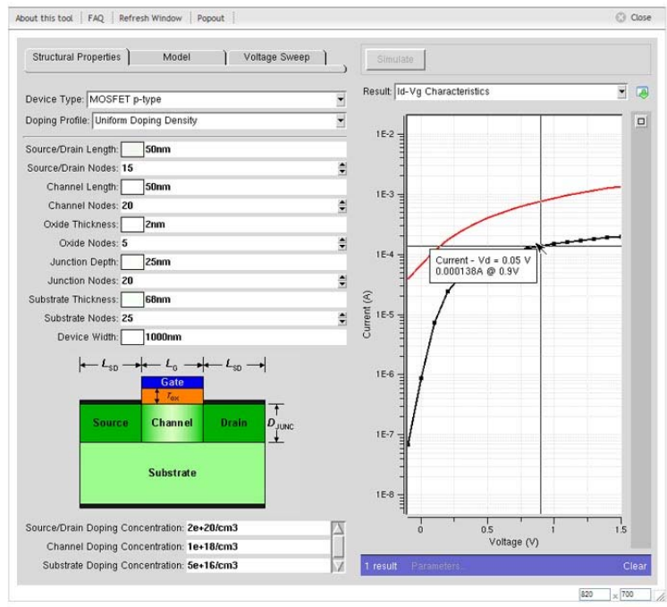
Figure 7: MOSFET simulation tool interface.
