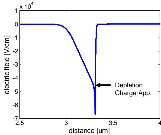
Figure 2. Electric field profile in a pn-diode with N_A=10^{16} \text{ cm}^{-3} and N_D=10^{18} \text{ cm}^{-3} and equilibrium conditions.
