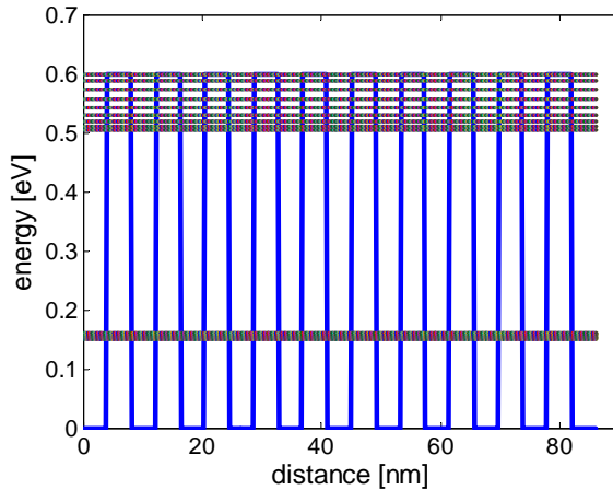
Figure 4. Multiple-barrier case and formation of energy bands due to the interaction between the wells.
