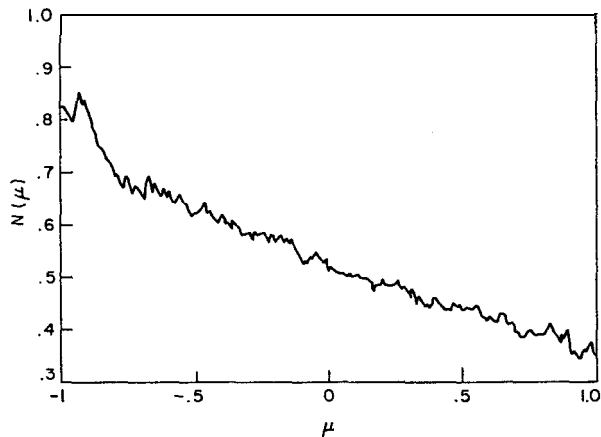
FIG. 12. Distribution function N(\mu) for \mu = \cos\theta_I , defined by Eq. (4.13). The decline with increasing \mu indicates a tendency for \mathbf{y}_I^{(2)} and \mathbf{N}_I to be antiparallel.
