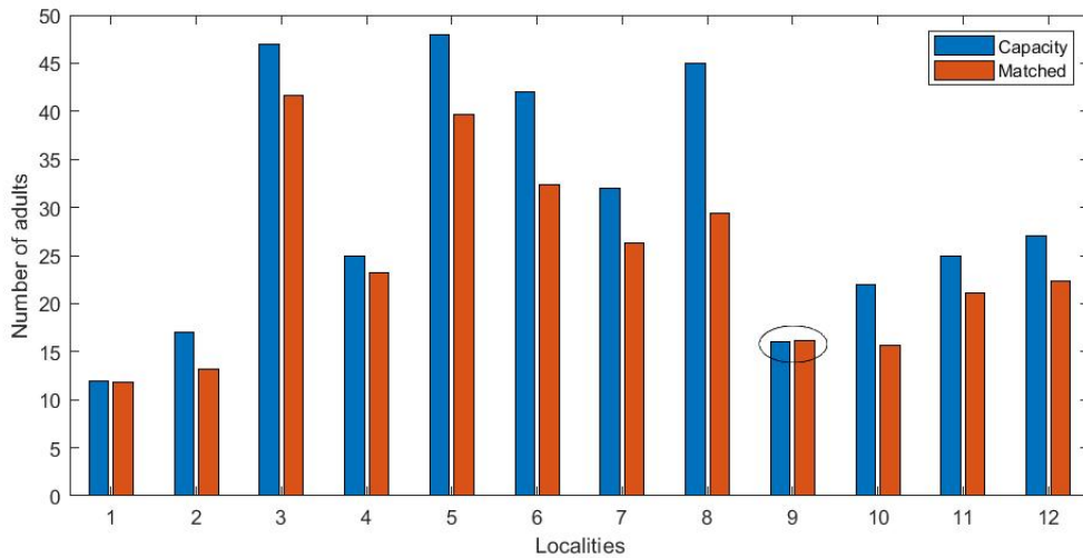
Figure 3: Average capacity under IR algorithm vs. actual capacity across all localities (number of adults constraint). Circles indicate localities where the constraint on the number of adults was violated on average.
