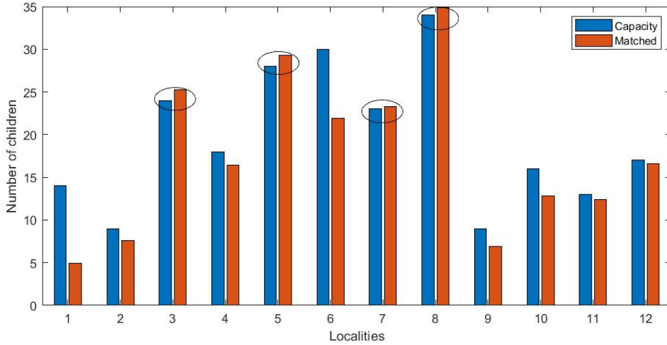
Figure 2: Average capacity under IR algorithm vs. actual capacity across all localities (number of children constraint). Circles indicate localities where the constraint on the number of children was violated on average.
