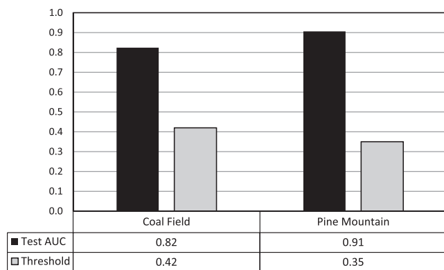
Fig. 4. Area under the curve (AUC) and presence–absence threshold determined for hemlock distribution models in two physiographic regions generated from MaxEnt.
