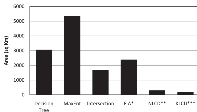
Fig. 3. Area (km 2 ) predicted as eastern hemlock by each modeling technique. Intersection denotes the areas in which all three models predict the presence of eastern hemlock. *Total forested area on which one or more hemlock trees occur based on Forest Inventory and Analysis data. **National Land Cover Dataset (NLCD) shows the total area classified as evergreen forest. ***Kentucky Anderson Level III Land Cover Dataset (KLCD) shows the total area classified as hemlock forest and hemlock-mixed deciduous forest.
