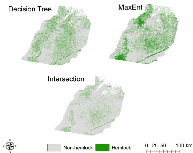
Fig. 2. Predicted distribution of eastern hemlock resulting from two modeling approaches, decision tree and MaxEnt (see text for full explanation). Intersection denotes the areas in which both models predict the presence of eastern hemlock.
