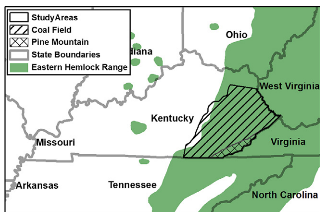
Fig. 1. Study area in relation to the range of eastern hemlock (Little, 1971), with the two physiographic regions, Coal Field and Pine Mountain, shown.
